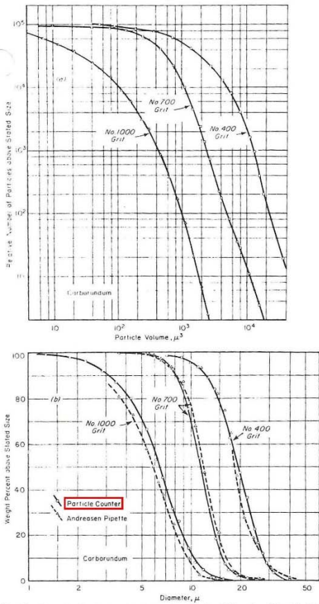
FIG. 5.—Narrowly Sized Abrasive Grades Suitable for Calibration, Plotted with Comparative Sedimentation Data.
