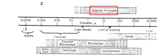
FIG. 2.—Size Range of Electric Method Compared with Coverage of Sieve, Sedimentation, and Microscope Methods, and Overlap of Electron Microscope and Centrifuge Ranges.
